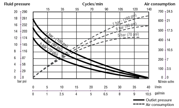
SAE 30 - 20 °C CAPACITY CURVE
